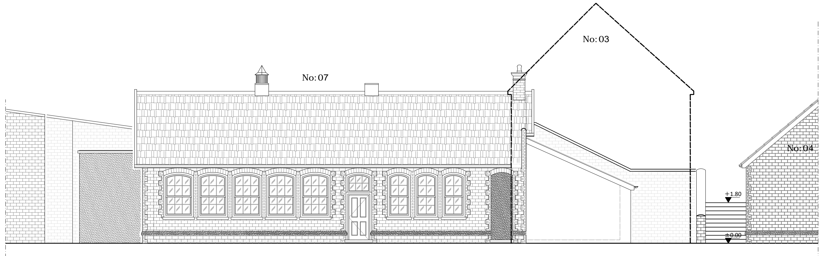
EXISTING FRONT ELEVATION SCALE: 1/100
