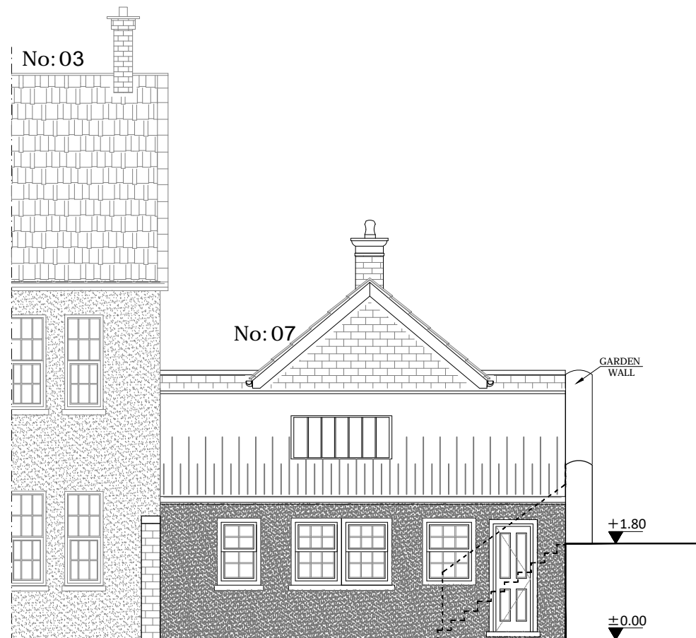
EXISTING SIDE ELEVATION SCALE: 1/100
